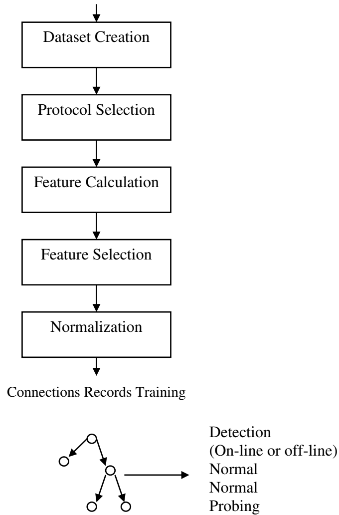
Figure 3.5: The stages of pre-processing data [24].
